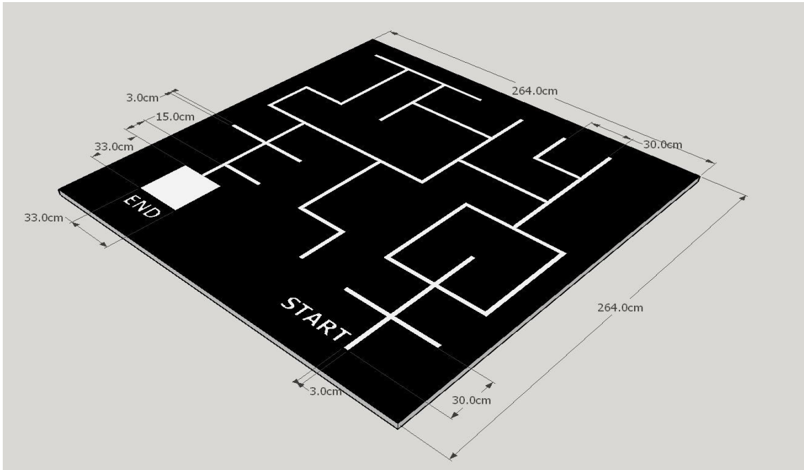
Fig. 1 Top View
