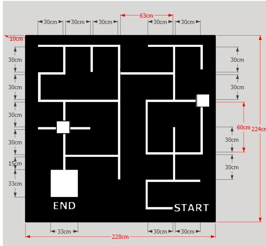
Fig. 1 Top View
