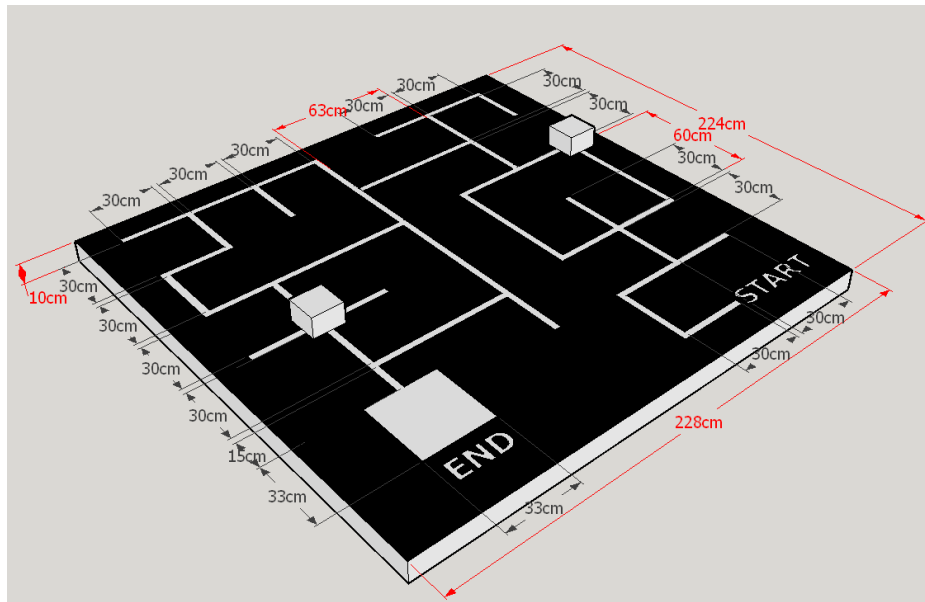
Fig. 2 Isometric View
